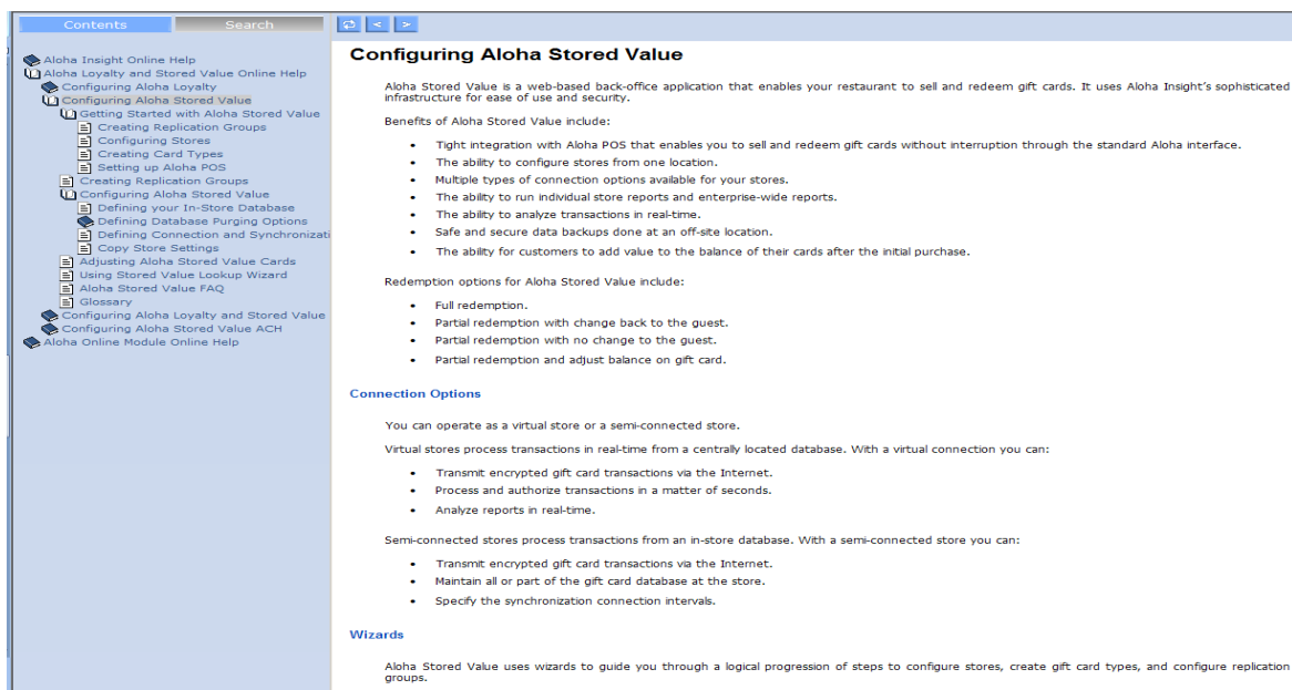
Figure 5 – Online Help
